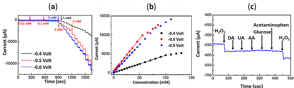
Fig. 3. (a) The amperometric response (i-t curve) of the GPS electrode, (b) The calibration curves corresponding to the data of (a) upon successive addition of \text{H}_2\text{O}_2 at various potentials of -0.4 \text{ V} to -0.6 \text{ V} in 0.1 M PBS (pH = 7.2). (c) The i-t curves for the interference studies of GPS with the presence of interfering species of 0.1 mM DA, UA, AA, acetaminophen, and 5 mM glucose at -0.5 \text{ V} .
