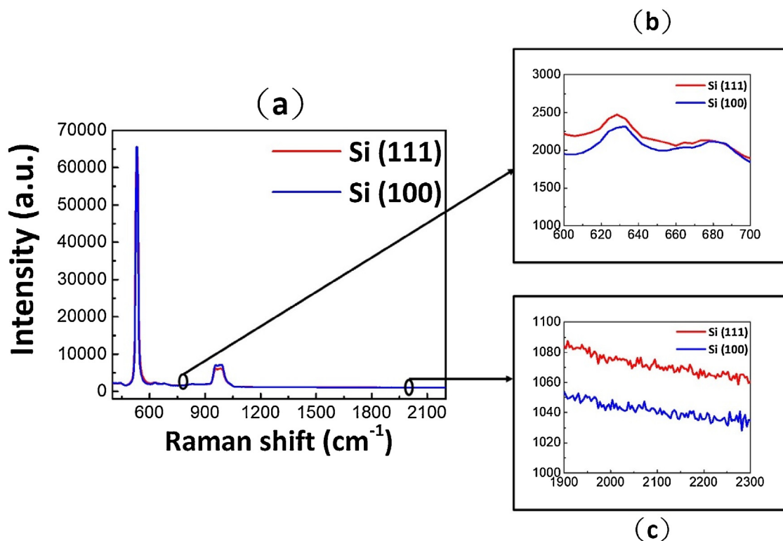
Fig. 6. The Raman spectra of Si (100) and Si (111) (a). The zoom-in comparison of Si—H bonds at 630 cm -1 (b) and 2000 cm -1 (c).
