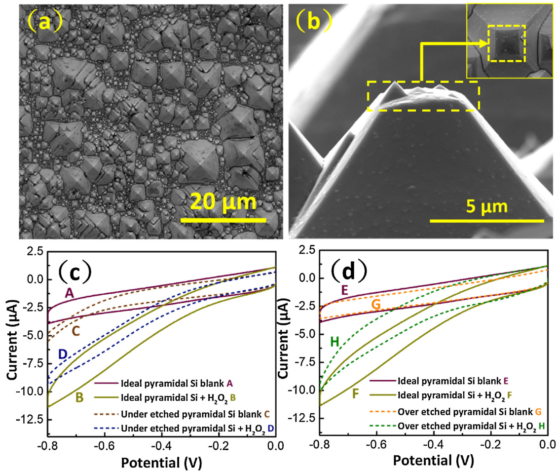
Fig. 4. SEM images of (a) the under-etched (15 min) and (b) the over-etched pyramidal Si (35 min). The inset in (b) is the top view of the over-etched pyramids. The cyclic voltammograms (CVs) of under-etched (c) and over-etched (d) Si electrodes in comparison with ideal pyramidal Si (111). The tests were conducted in the absence (the “blank” denotation of A, C, E, and G curves) and presence of 5 mM H 2 O 2 (B, D, F, and H curves) in 0.1 M PBS (pH = 7.2) with a scan rate of 50 mV s -1 .
