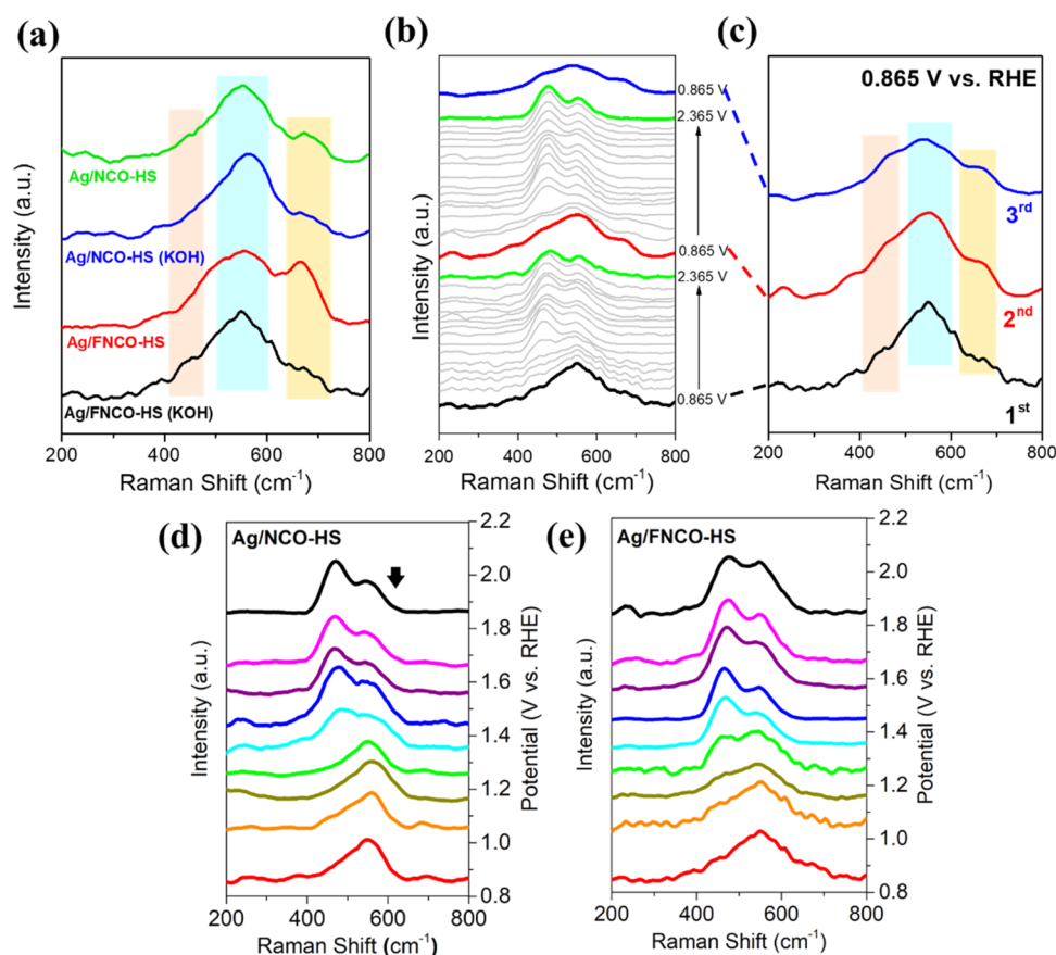
Figure 6. Raman studies of the electrocatalysts. (a) Comparison of Ag/NCO-HS and Ag/FNCO-HS in dry and KOH-immersed conditions. (b) Raman spectra of Ag/FNCO-HS associated with the charge–discharge OER cycles: charging from 0.865 to 2.365 V (black to green) and then return to the rest conditions at 0.865 V immediately (green to red). (c) Comparison of zero charge (0.865 V) curves acquired from (b) connected with the dashed lines. The notation of 1st, 2nd, and 3rd represents the rest conditions between two successive charge–discharge cycles. The pink, blue, and yellow highlights in (a) and (c) emphasize the Raman shift bands of 450, 550, and 670, cm -1 , respectively. Operando Raman-coupled electrocatalysis of (d) Ag/NCO-HS and (e) Ag/FNCO-HS during the OER process; the arrow in (d) indicates the shoulder for the Co III OOH vibration. The right axes show the potential at which each Raman spectrum was measured.
