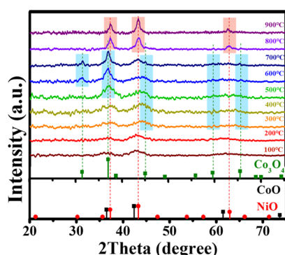
Figure 2. Phase transformation of NCO-HS monitored by XRD at a calcination temperature range from 100 to 900 °C. The \text{Co}_3\text{O}_4 phase occurs from 300 °C and then disappears at 800 °C (see the blue bar labels). The co-existing NiO and \text{Co}_3\text{O}_4 phases change into a single phase as the temperature reaches 800 °C, corresponding to a rock salt CoO–NiO solid solution of NCO-HS.
