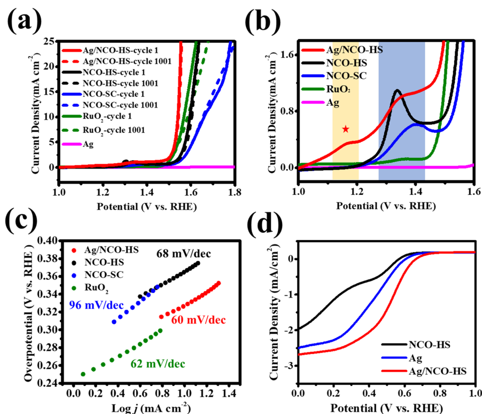
Figure 4. Electrocatalytic performance comparison. (a) OER LSV curves of the samples in 0.1 M KOH at a rotation of 1600 rpm. (b) The magnified OER LSV curves of (a) reveal the potentials for oxidation number changes of Ni and Co in the electrocatalysts. Two peak regions labeled by yellow and blue correspond to Co and Ni oxidation signals, respectively. (c) OER Tafel plots of the electrocatalysts. (d) ORR LSV curves of the samples recorded at 1600 rpm in O 2 -saturated 0.1 M KOH (counter electrode: glassy carbon).
