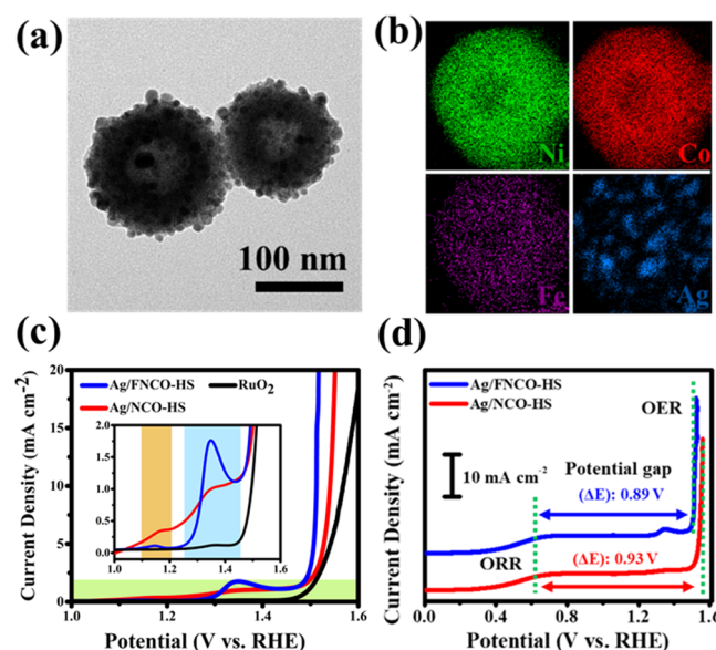
Figure 5. Characterization of Ag-decorated Fe-doped NiO–CoO hollow spheres (Ag/FNCO-HS). (a) TEM images of Ag/FNCO-HS. (b) EDS mapping of Ni, Co, Fe, and Ag of an individual hollow sphere. (c) OER LSV curves catalyzed by Ag/FNCO-HS in comparison with iron-free Ag/NCO-HS; the inset, which magnifies the green region, shows the peaks corresponding to \text{Co}^{2+} (orange band) and \text{Ni}^{2+} (light blue band) oxidation. (d) ORR and OER bifunctional activities of Ag/FNCO-HS with a potential gap smaller than Ag/NCO-HS by 40 mV.
