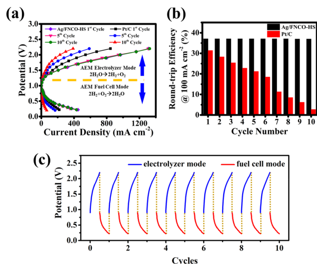
Figure 8. Comparison of the performance of AEM devices between electrolyzer and fuel cell modes using Ag/FNCO-HS and Pt/C. (a) Polarization curves of the devices measured over 10 cycles, where each cycle includes one electrolyzer test, followed by one run of the fuel cell mode. (b) Round-trip efficiency (based on eq 1) at 100 \text{ mA cm}^{-2} for 10 cycles. The carbon-free Ag/FNCO-HS shows higher durability than carbon-based Pt/C. (c) Data set of the cycle tests, where the yellow dotted lines indicate the swapping in each cycle. The maximum current densities achieved are 1.3 \text{ A cm}^{-2} and 430 \text{ mA cm}^{-2} for the electrolyzer and fuel cell modes, respectively.
