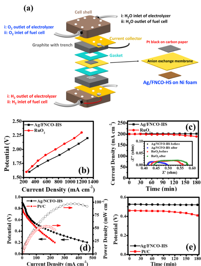
Figure 7. Bifunctional device performance using the Ag/FNCO-HS catalyst as compared to the benchmarks. (a) Cell assembly of the AEM device where the inlets and outlets for electrolyzer and fuel cell modes are labeled (i) and (ii), respectively. (b) Electrolyzer mode performance comparison between Ag/FNCO-HS and \text{RuO}_2 as alkaline OER electrocatalysts. (c) Corresponding stability tests of catalysts in (b) at a constant potential of 1.50 V, where the inset shows the EIS of the corresponding devices measured before and after the stability tests. (d) Fuel cell mode performance comparison between Ag/FNCO-HS and Pt as the alkaline ORR electrocatalysts. (e) Stability tests of the catalysts in (d) at a constant current density of 100 \text{ mA cm}^{-2} .
