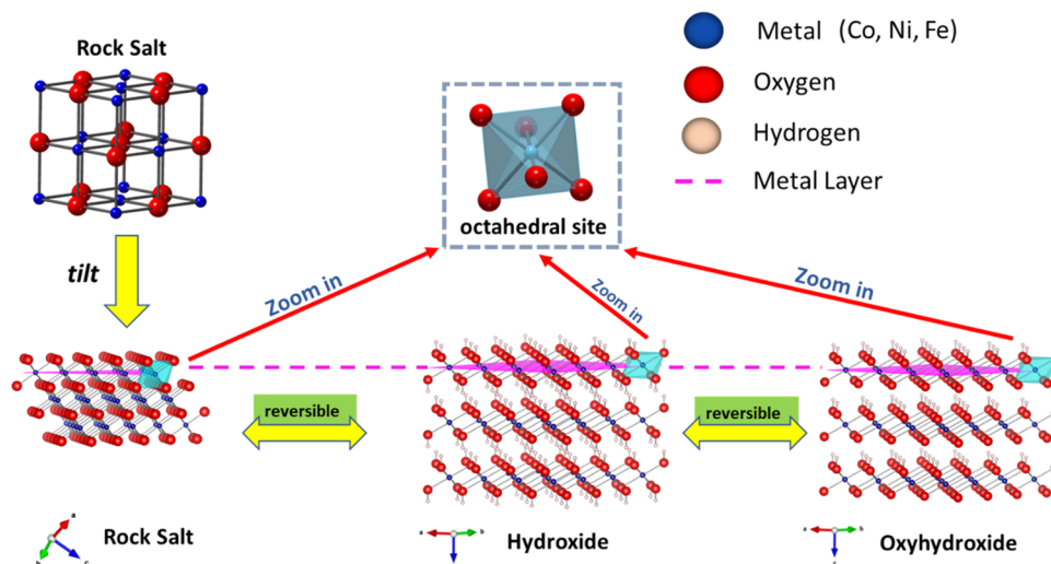
Scheme 2. Illustrated Phase Transition of Rock Salt Ternary Oxides during the OER Process a
