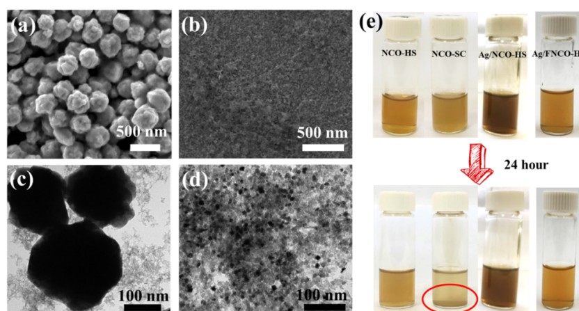
Figure 3. Characterization of control samples and suspension tests. (a) SEM and (c) TEM images of the samples prepared using the oleylamine-free procedure yielding solid-core samples (NCO-SC). (b) SEM and (d) TEM images of the samples prepared using a TBAOH-free procedure showing nanoflakes instead of a spherical morphology. (e) Suspension tests of NCO-HS, NCO-SC, Ag/NCO-HS, and Ag/FNCO-HS in a water/IPA solution. After 24-h aging, all of the hollow structure samples remain well suspended, except for NCO-SC (precipitates are indicated by the red circle).
