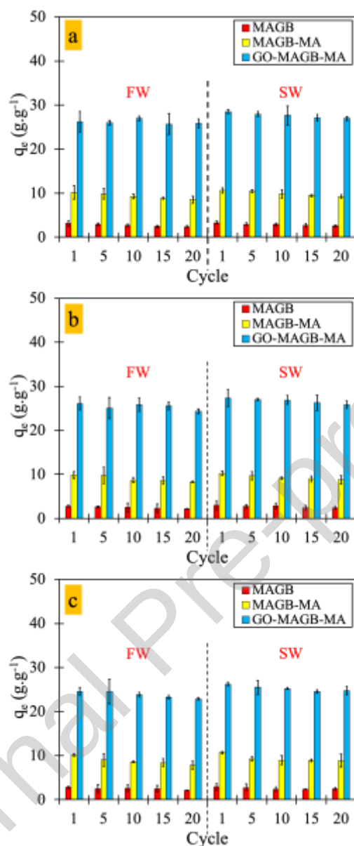
Fig. 9. Recycle test of MAGB, MAGB-MA and GO-MAGB-MA for magnetic removal of oil in freshwater (FW) and seawater (SW) at (a) 25 °C, (b) 35 °C, and (c) 45 °C (experiment condition: C_0 : 100 g.L -1 , t: 2 h, adsorbent dose: 1 g.L -1 and n: 3).
